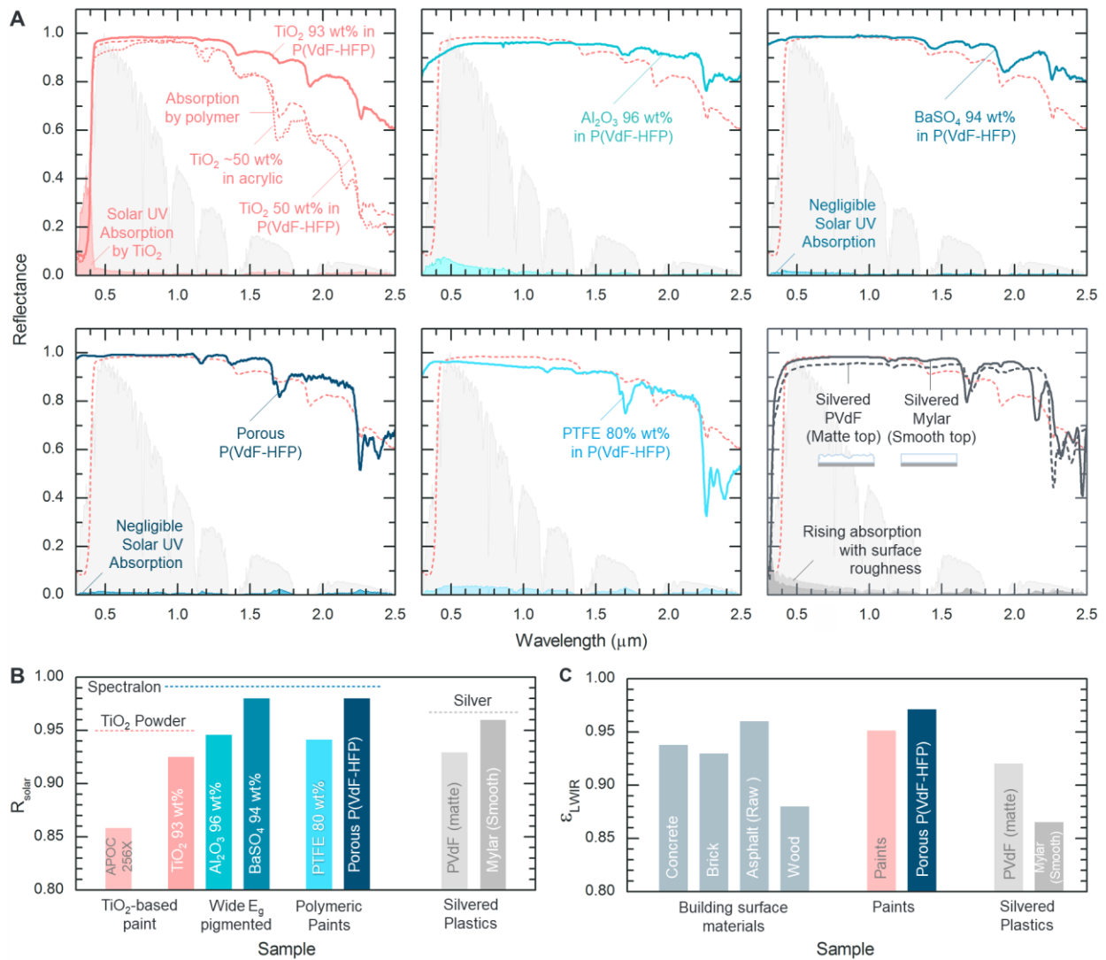
Figure 2. (A) (From top-left to bottom right) Measured spectral reflectances of paints based on TiO 2 , Al 2 O 3 , BaSO 4 , porous P(VdF-HFP) and PTFE, and silvered plastics. The paint films are all ~1 mm thick. (B) R_{\text{solar}} of paints and silvered plastics. APOC 256X paint is rated by the Cool Roof Rating Council as the most reflective on the market. The dotted lines show the reflectances of TiO 2 powder, spectralon (porous PTFE), and silver, and represent the likely upper limits of R_{\text{solar}} of TiO 2 -based, polymer-based, and silvered radiative coolers respectively. Note that the reflectances were weighted using ASTM G-173 solar spectrum, which assumes a solar zenith angle of 48.19°. During summertime or in the tropics, the noon-time zenith angle is smaller. Consequently, UV light is stronger and further lowers R_{\text{solar}} of TiO 2 and silver-based designs. (C) \epsilon_{\text{LWIR}} of common building materials, paints and silvered emitters.
