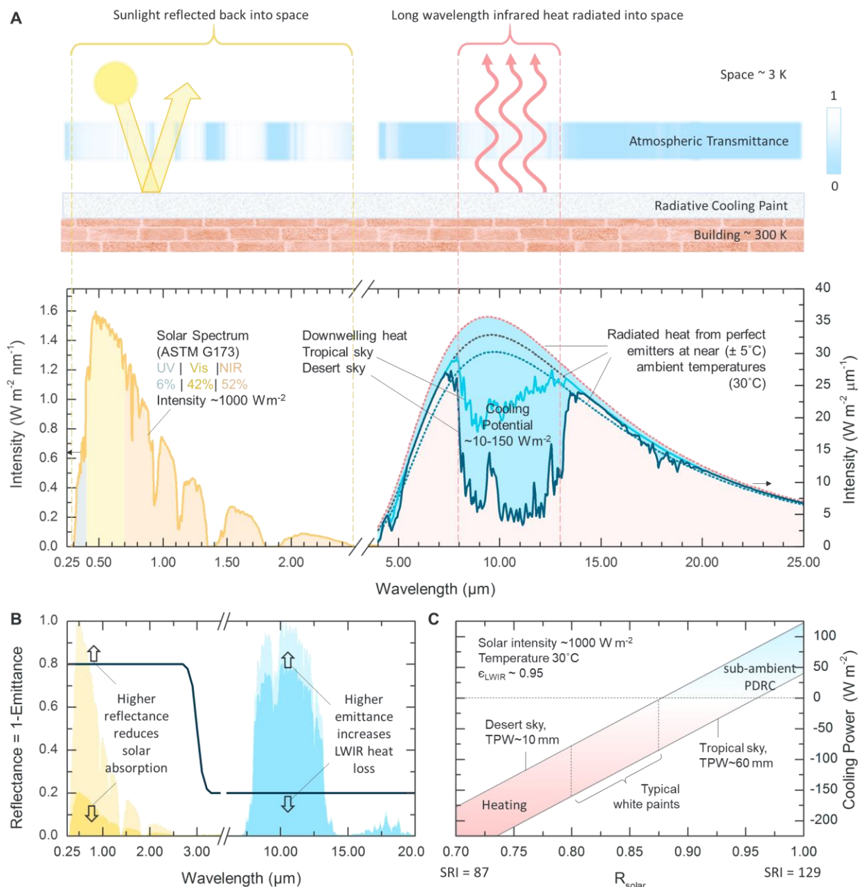
Figure 1. (A) Schematic showing passive daytime radiative cooling by solar reflection and LWIR thermal emission through the atmospheric transmission windows. Corresponding solar and thermal spectra are shown below. (B) Schematic showing how high solar reflectance and thermal emittance enable PDRC. It should be noted that at near-ambient temperatures, radiative transfer (= radiated heat from emitter – downwelling heat from sky) is small outside the LWIR window, making broadband and selective LWIR emitters similarly effective at cooling. (C) Schematic showing cooling powers (thermal emission – solar absorption) 1 of emissive coatings ( \epsilon_{\text{LWIR}} \sim 0.95 ) as a function of R_{\text{solar}} (or solar reflectance index (SRI), which varies linearly with R_{\text{solar}} ). R_{\text{solar}} > 0.95 usually yields sub-ambient radiative cooling.
